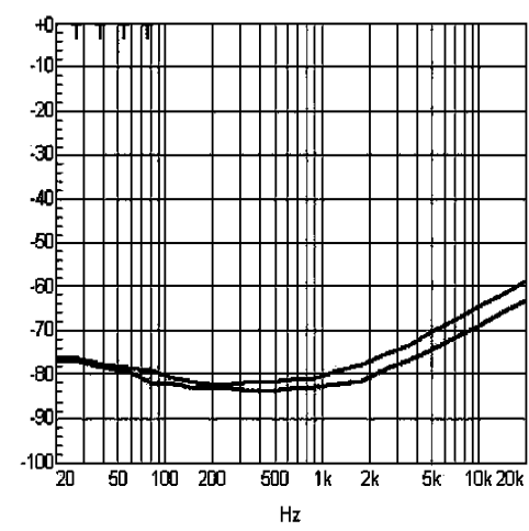
Figure 19 PSRR vs. Freq SE mode, 3V, 320Ohm, 200mVpp Input terminated
