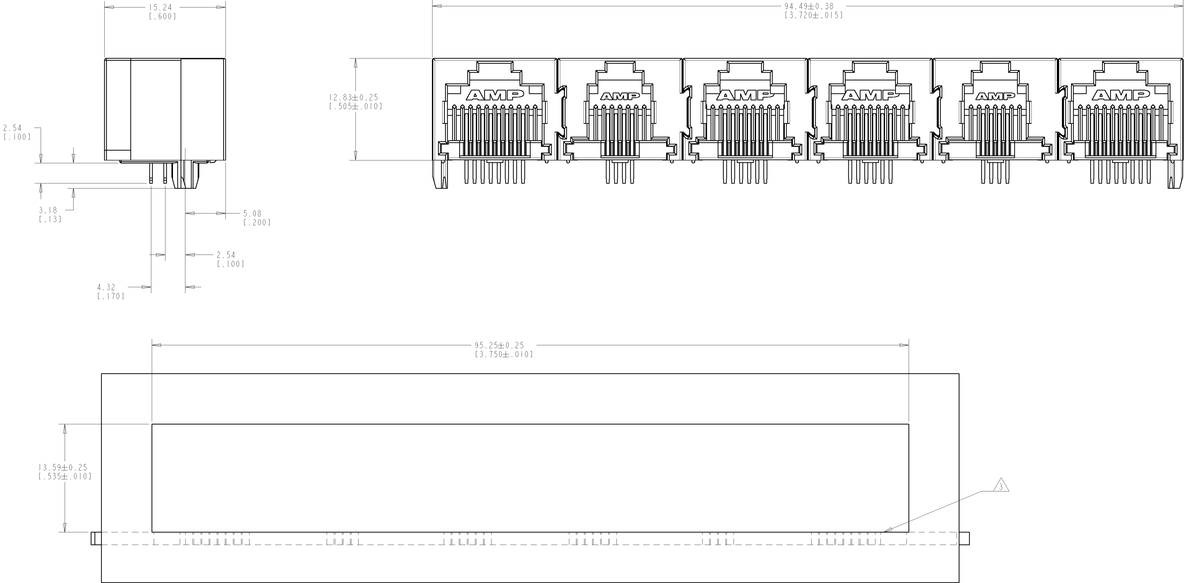
SUGGESTED PANEL OPENING SCALE 4:1
