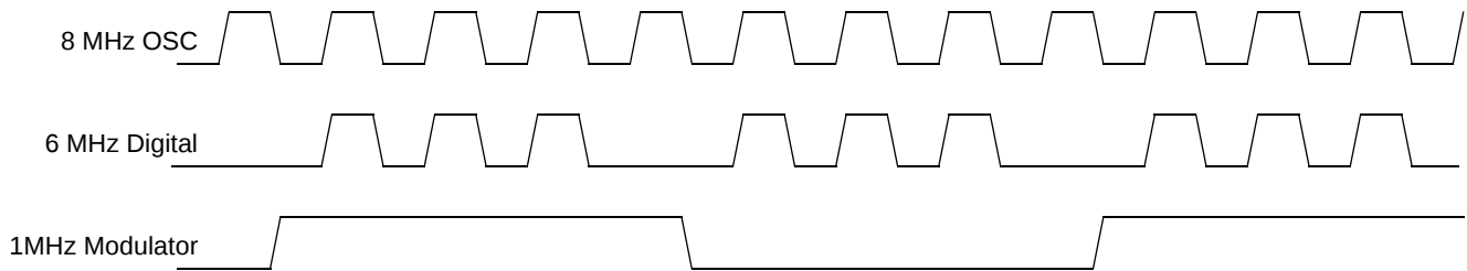
Figure 13. Clock Generation
