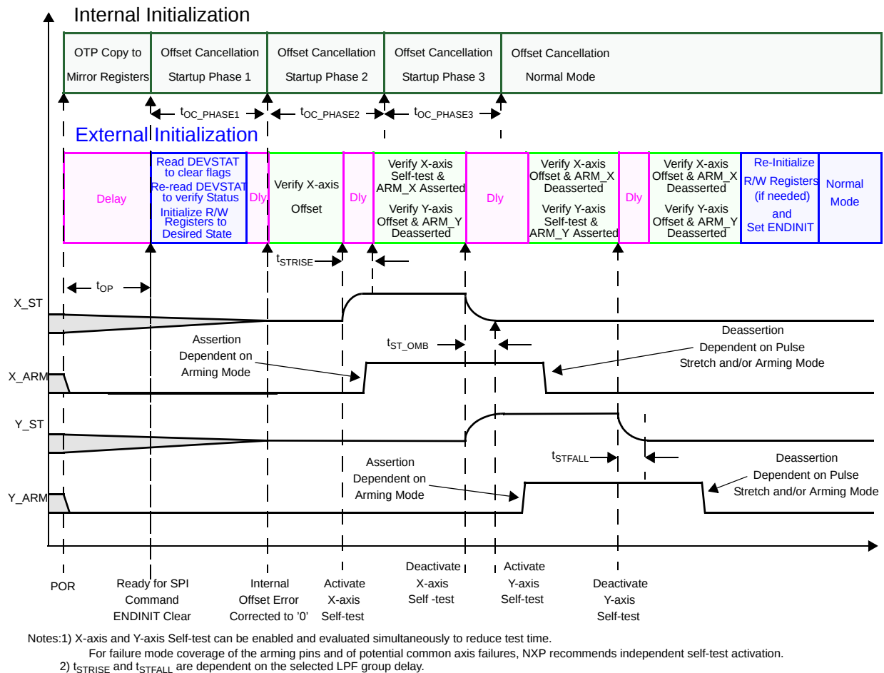
Figure 32. Initialization Process
