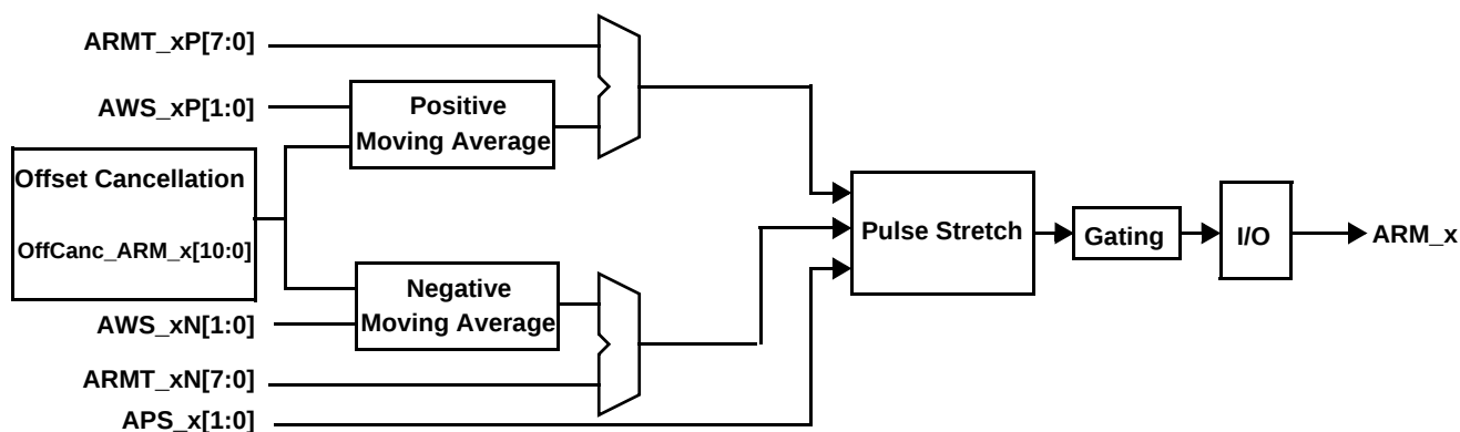
Figure 24. Arming Function Block Diagram - Moving Average Mode
