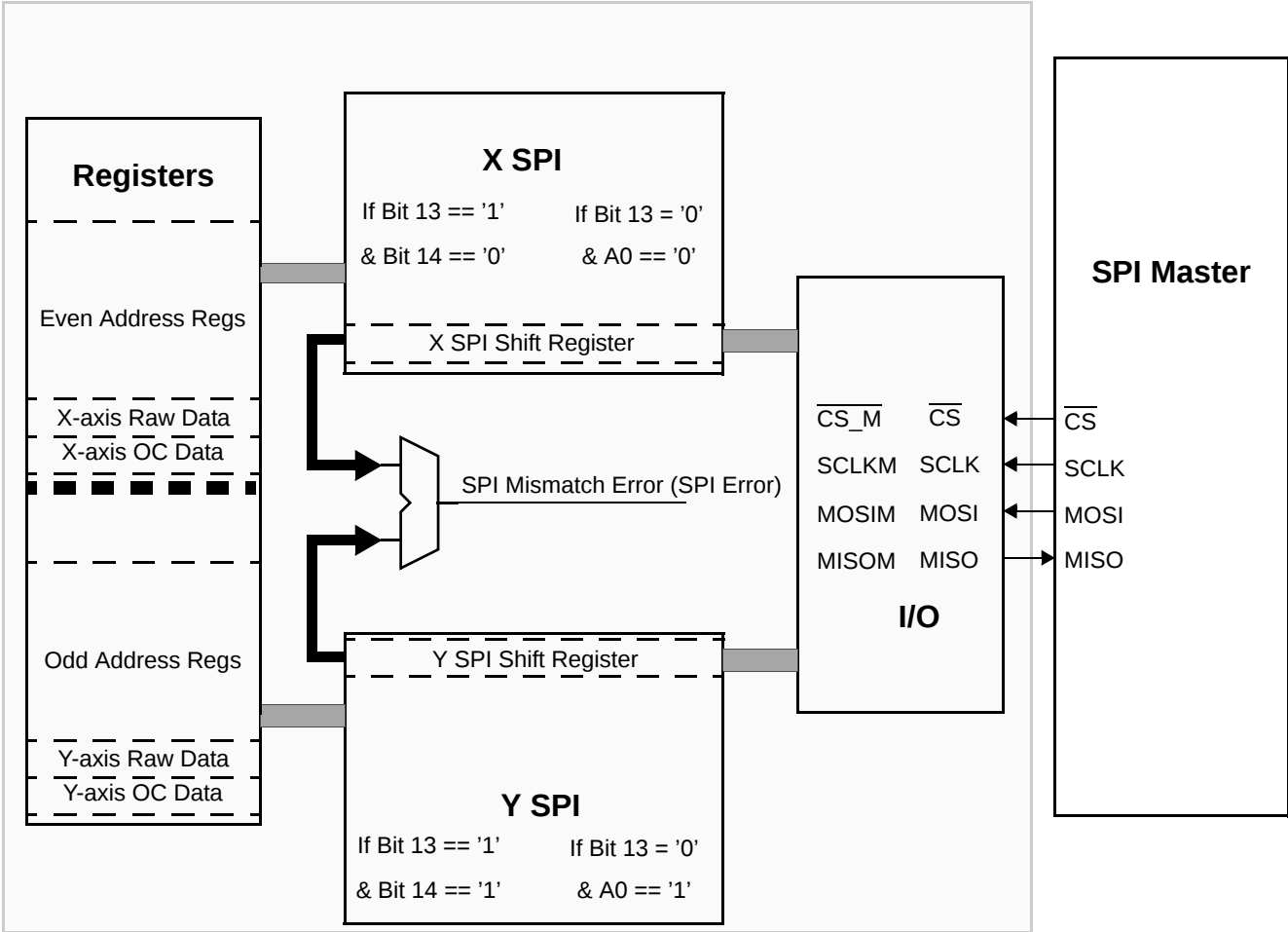
Figure 31. SPI Diagram
