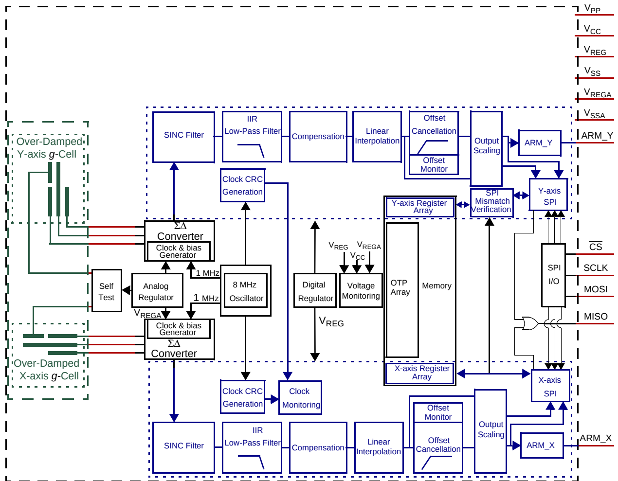
Figure 4. Block Diagram
