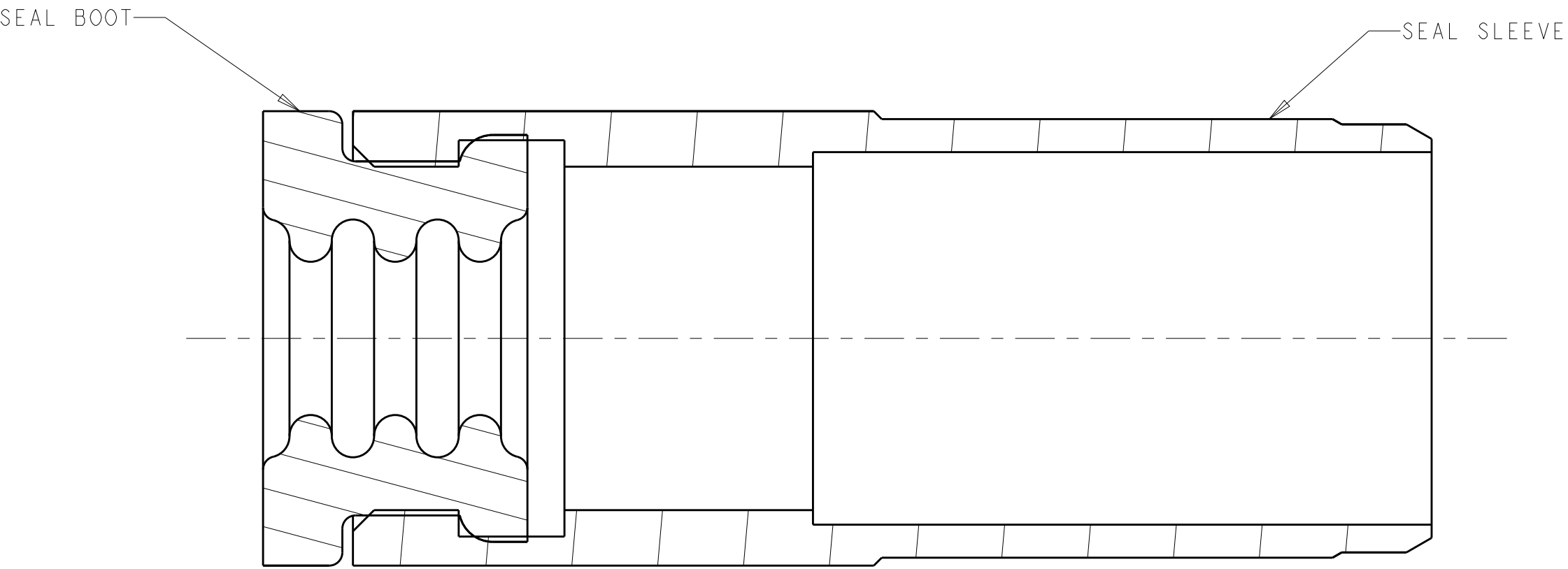
SECTION J-J
