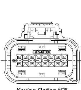
Keying Option "C" (Housing Color: Brown)
