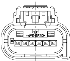
Keying Option "C"
