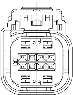
Keying Option "B"
