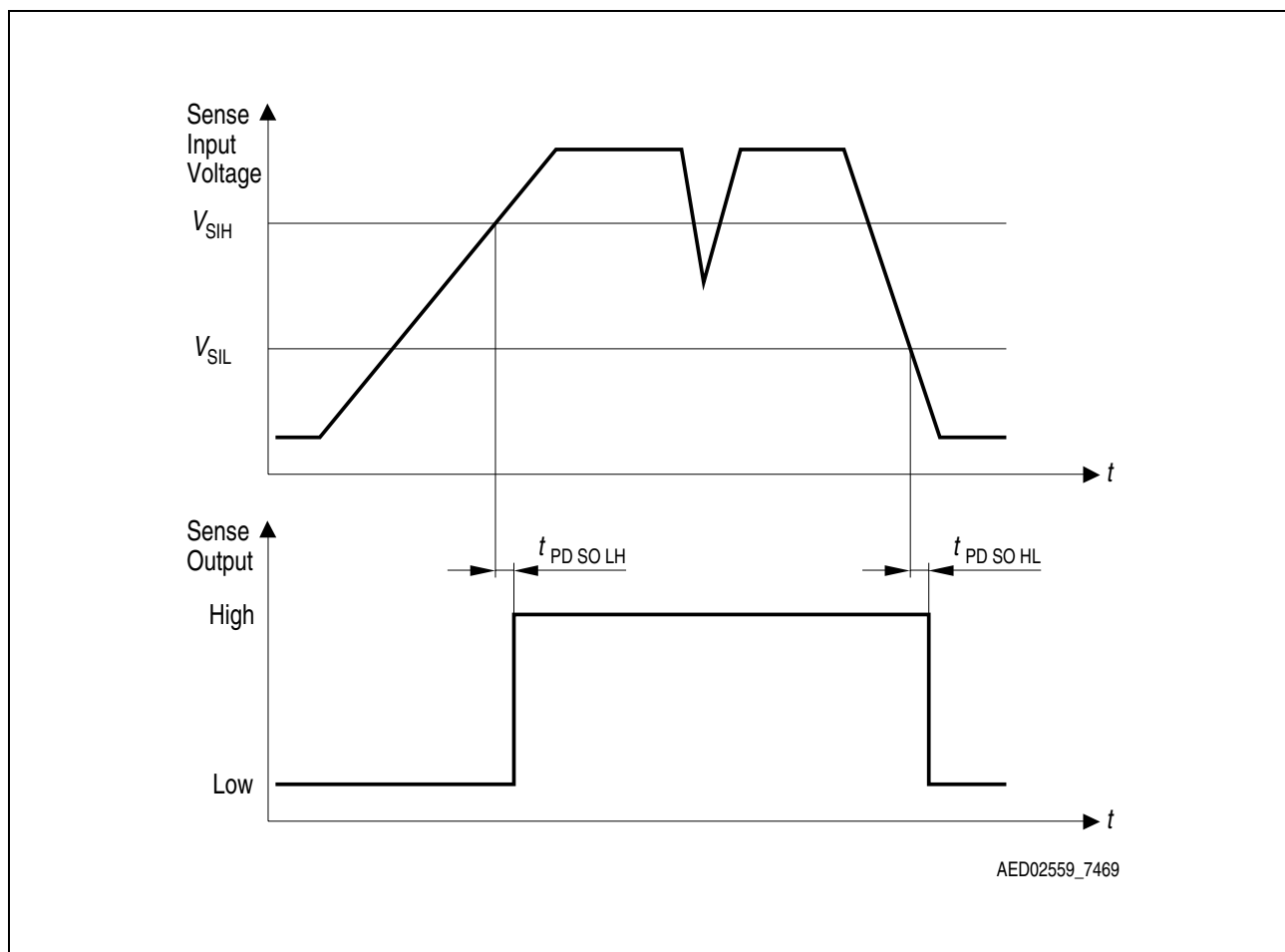
Figure 4 Sense Timing Diagram
