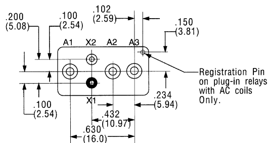
TERMINAL VIEW
