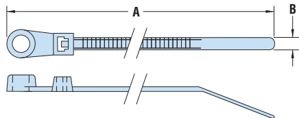
Screw Mount
