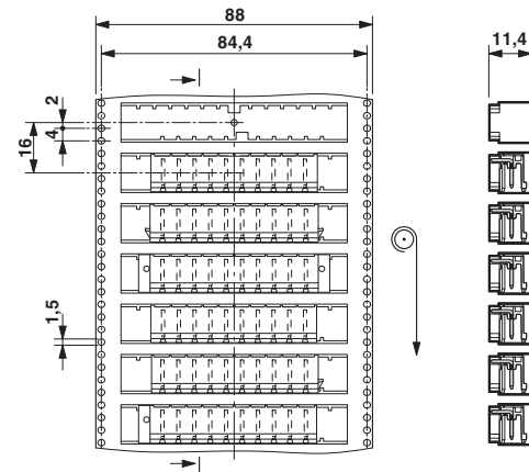
Dimensional drawing
