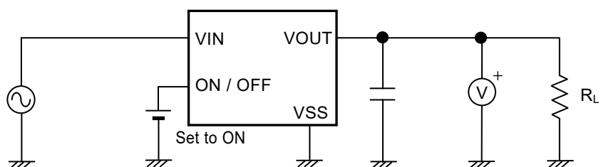
Figure 13 Test Circuit 5
