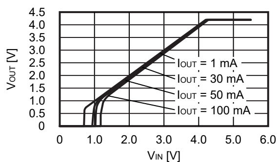
2.3 V_{\text{OUT}} = 4.2 \text{ V}
