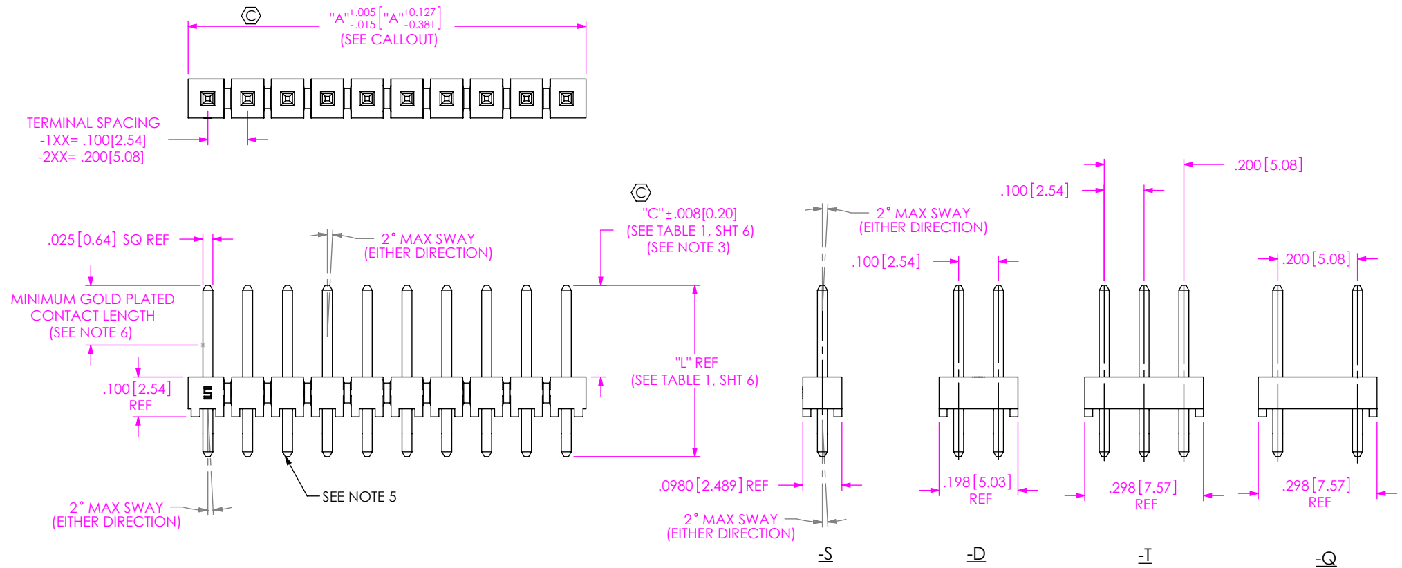
FIG 1 HTSW-110-07-XXX-D SHOWN
