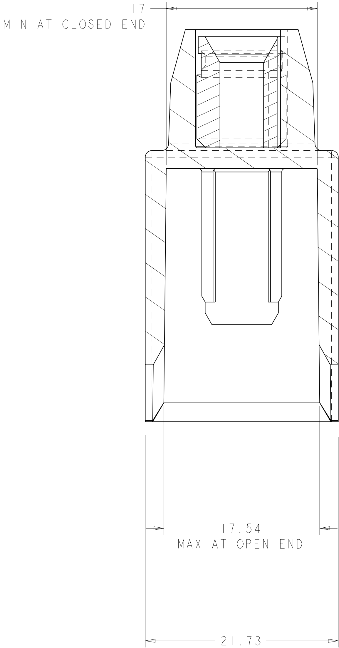
SECTION B-B
