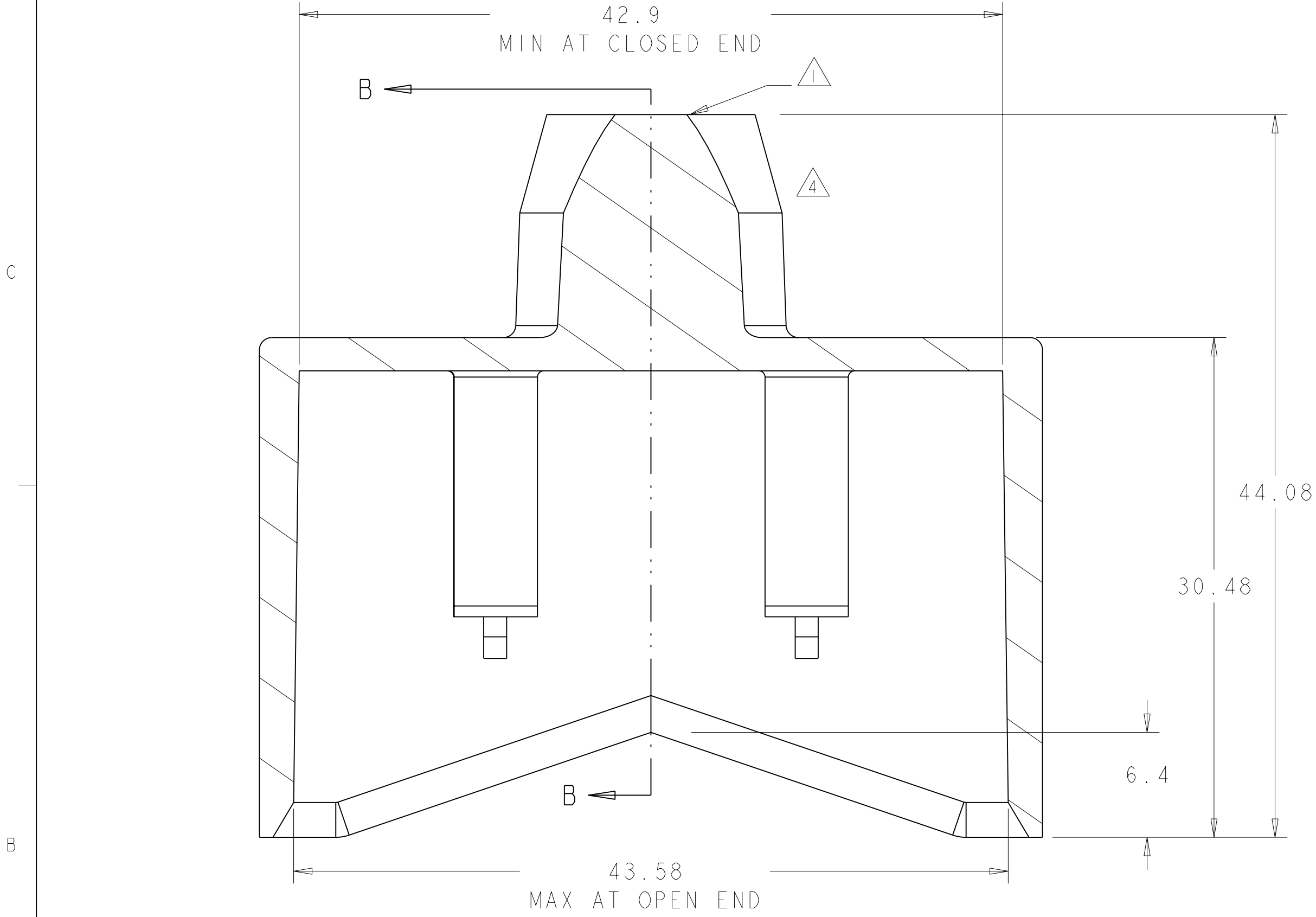
SECTION C-C
