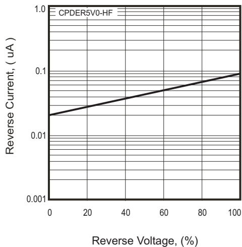
Fig.2-3 - Reverse Characteristics
