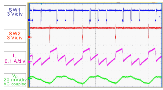
Figure 13. Buck-boost region operation @ I_O = 50\text{ mA}
