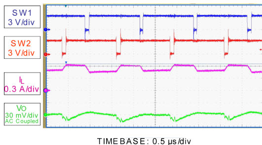
Figure 12. Buck-boost region operation @ I_O = 500\text{ mA}
