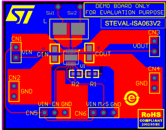
Figure 20. Component placement
