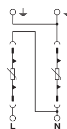
Circuit diagram
