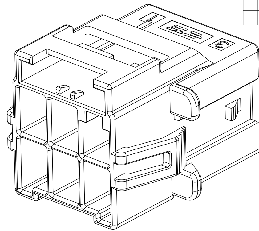
2*3 POSITIONS
