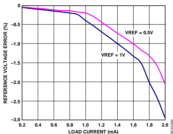
Figure 72. Reference Voltage Accuracy vs. Load Current
