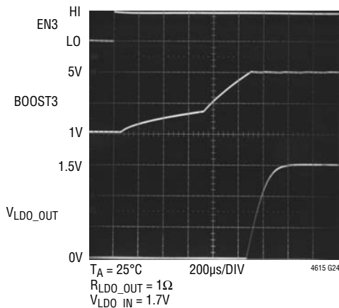
BOOST3/OUT Start-Up
