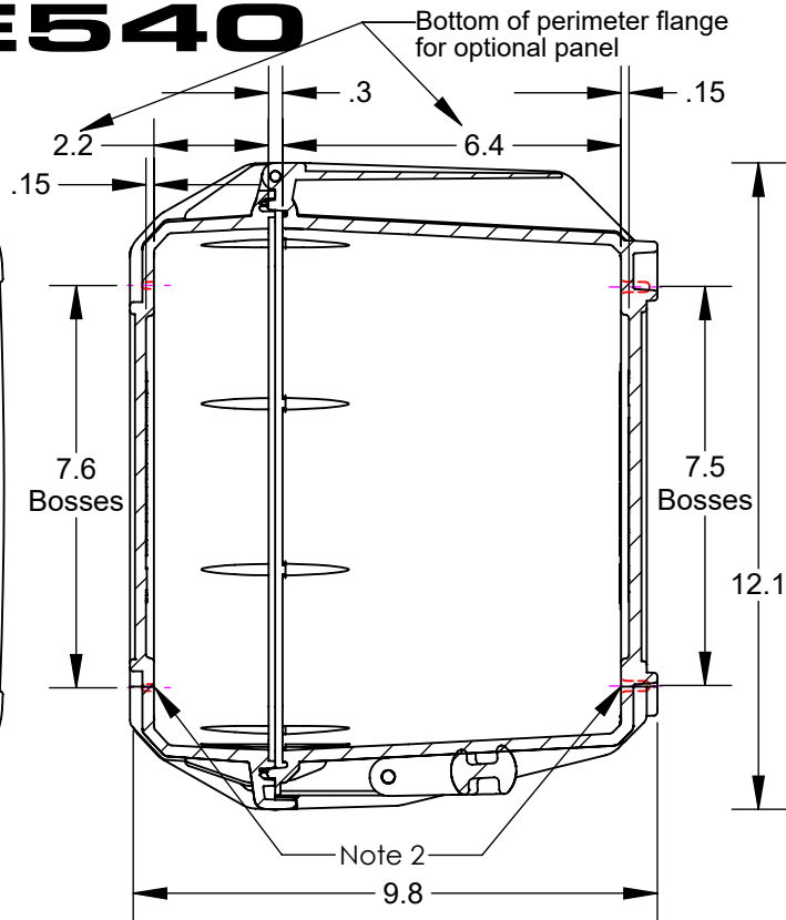
SECTION A_A
