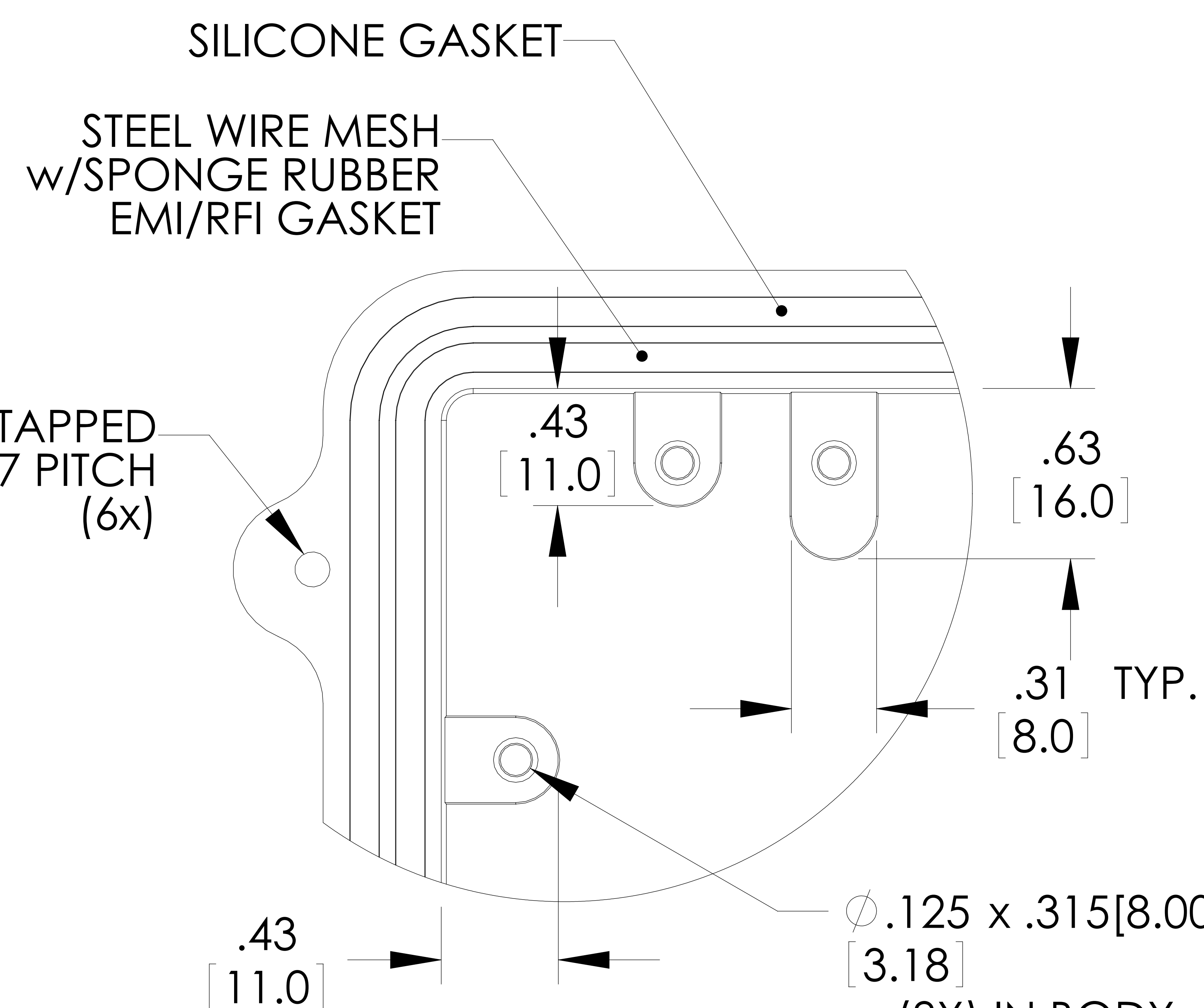
DETAIL B SCALE 4 : 1
