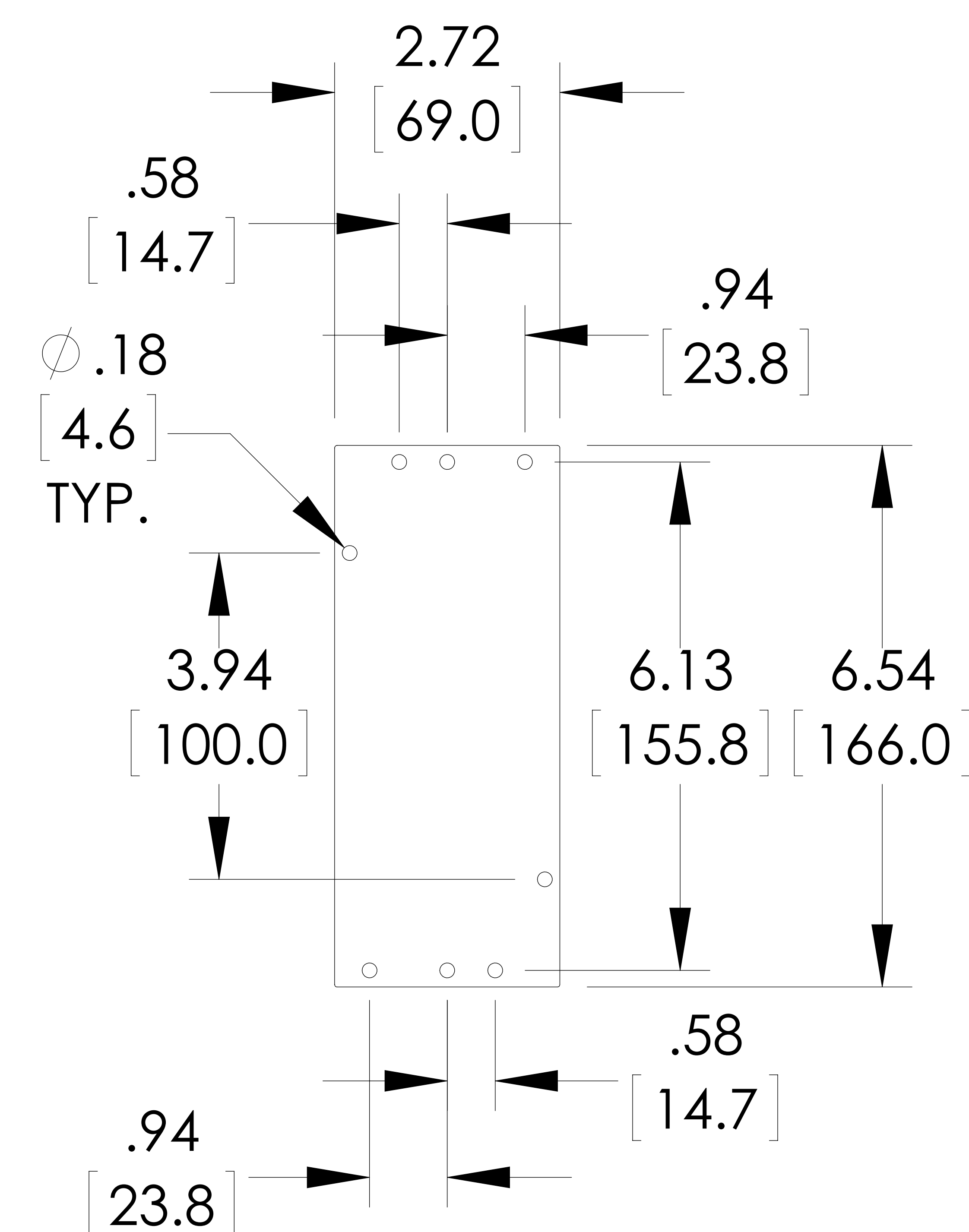
SUGGESTED PC BOARD OR INTERNAL PANEL LAYOUT
