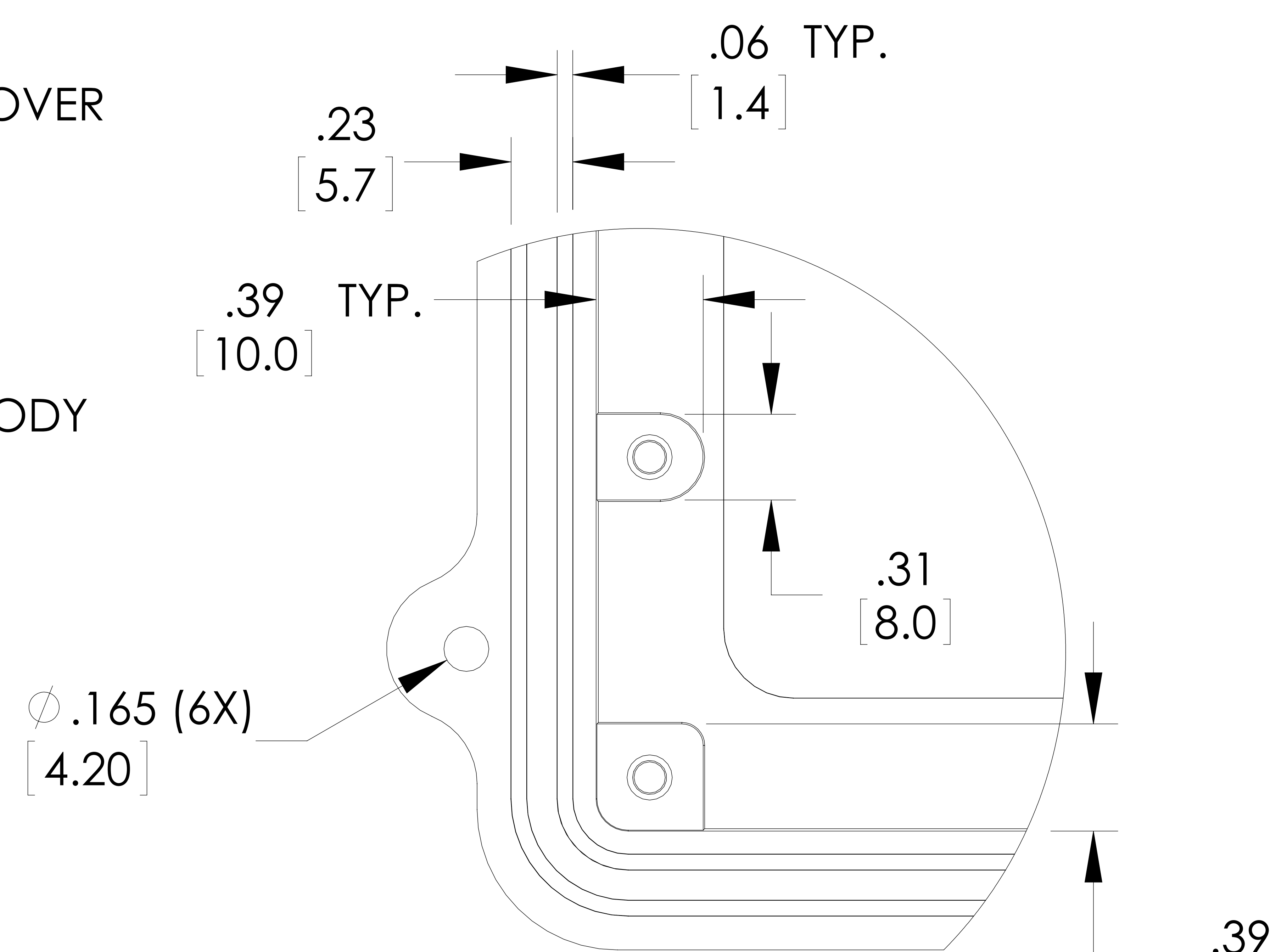
DETAIL C SCALE 4 : 1
