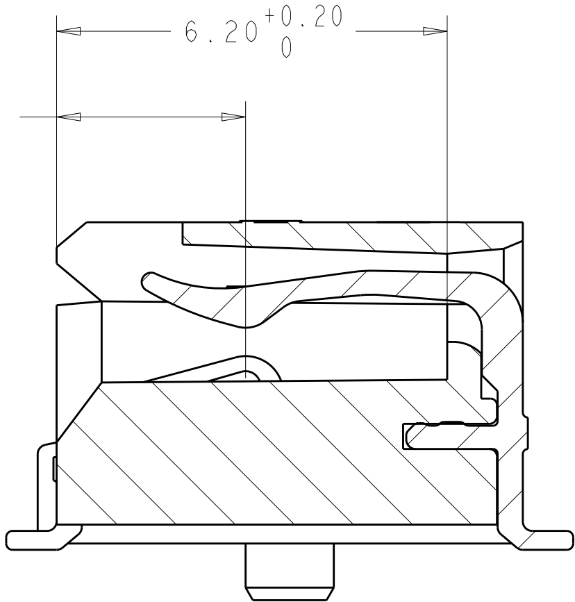
SECTION X-X
