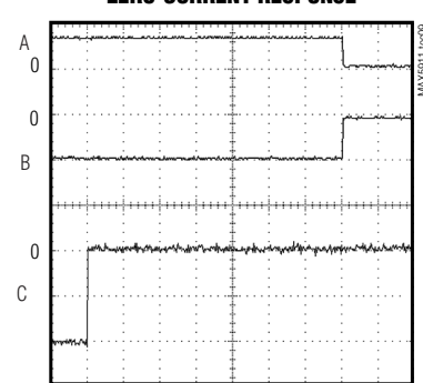
MAX5911 ZERO-CURRENT RESPONSE
