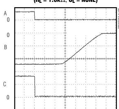
MAX5911 TURN-OFF WAVEFORMS ( R_L = 1.8k\Omega , C_L = \text{NONE} )
