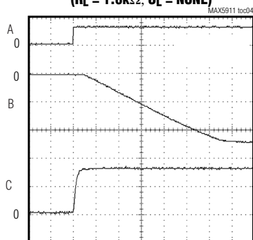
MAX5911 TURN-ON WAVEFORMS ( R_L = 1.8k\Omega , C_L = \text{NONE} )
