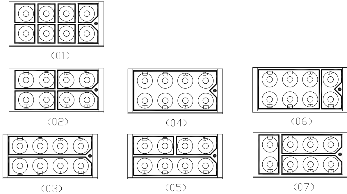
BUSSING ARRANGEMENTS
