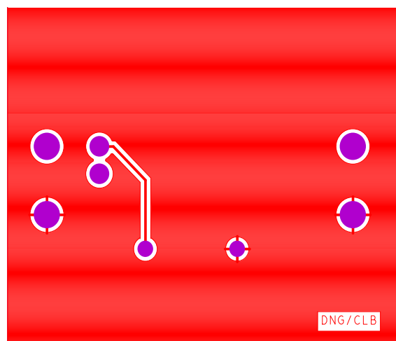
FIGURE 3. BOTTOM LAYER
