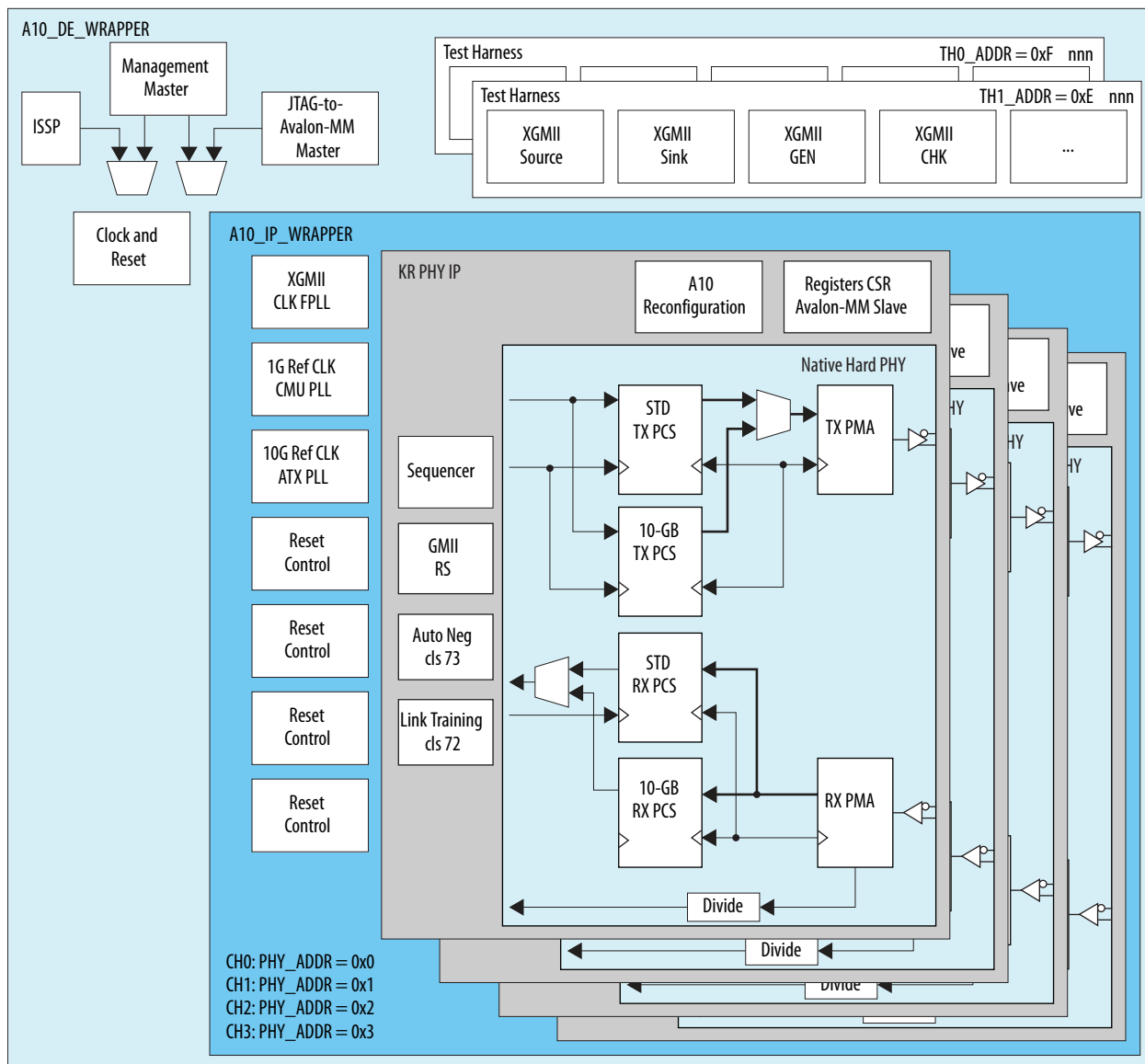
Figure 5-5: PHY-Only Design Example with Two Backplane Ethernet and Two Line-Side (1G/10G) Ethernet Channels
