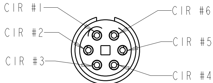
INSERT SUB-ASSY CIRCUIT DESIGNATION VIEW
