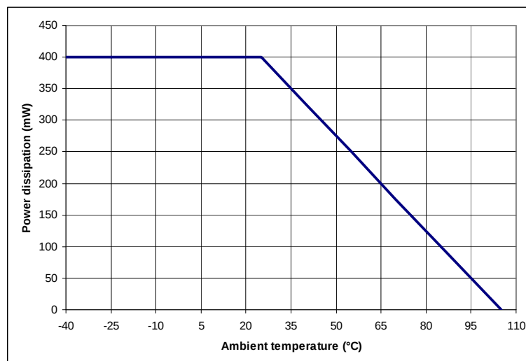
Figure 8 Derating Curve
