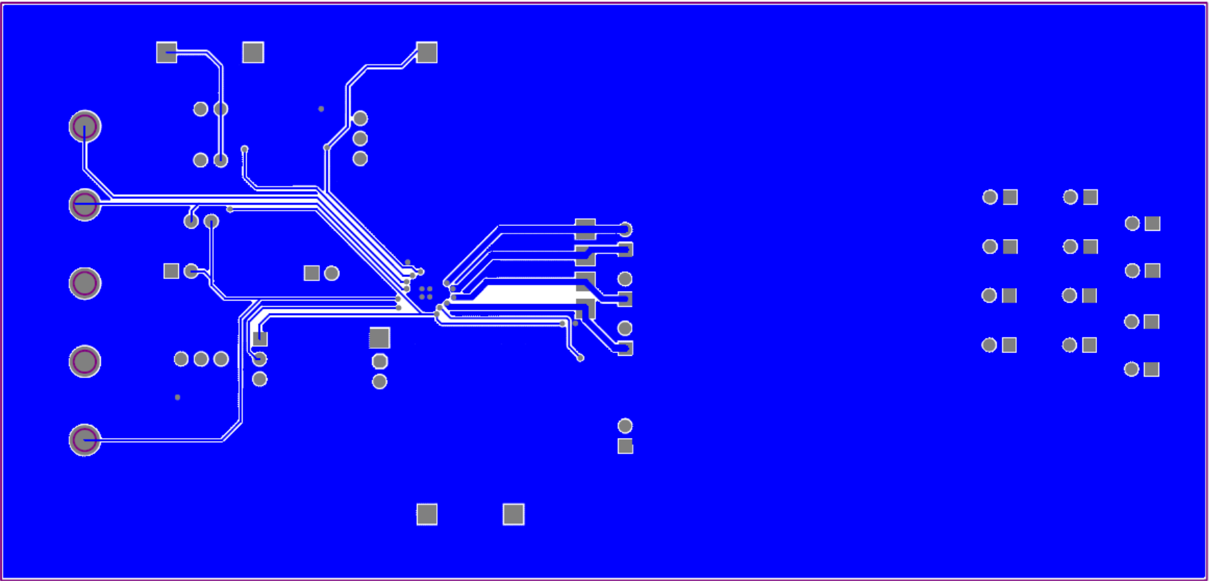
FIGURE 3. BOTTOM LAYER
