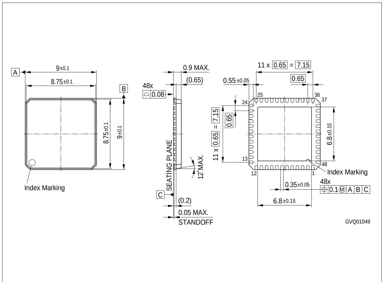
Figure 14 PG-VQFN-48
