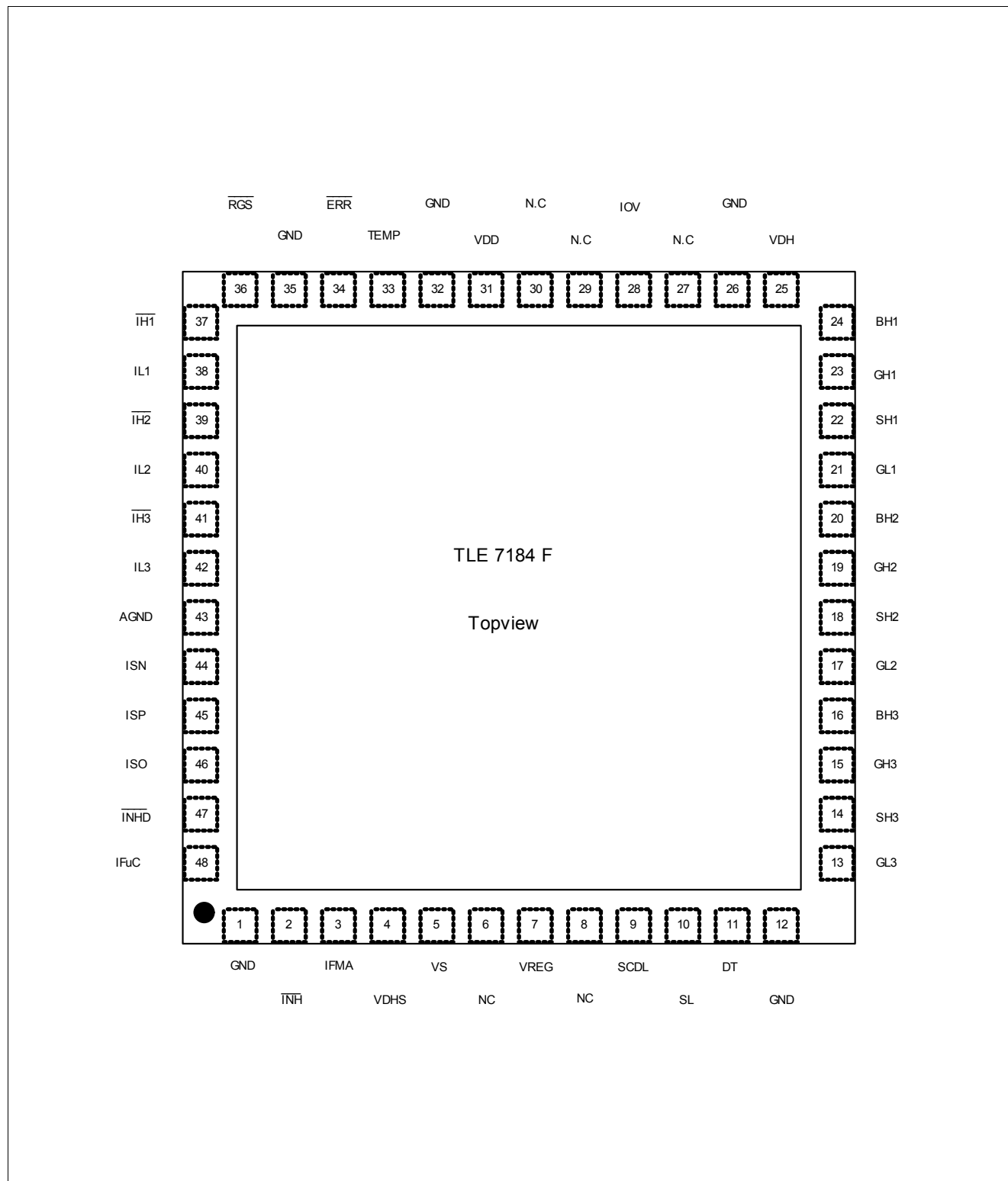
Figure 2 Pin Configuration
