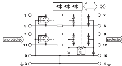
Application drawing
