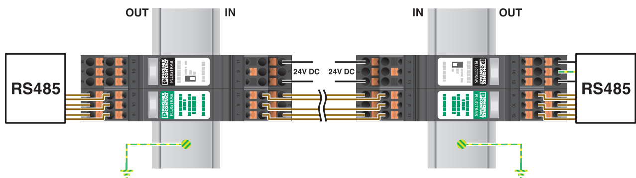
Application drawing
