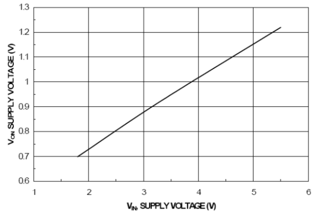
Figure 8. V_{O1} High Voltage vs. Input Voltage
