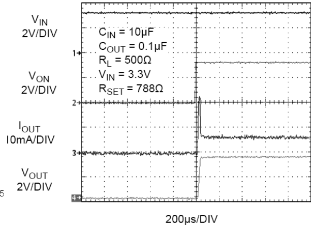
Figure 18. t_{ON} Response
