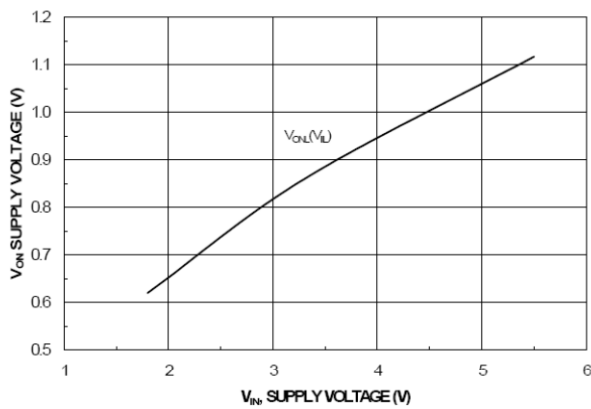
Figure 9. V_{O1} Low Voltage vs. Input Voltage
