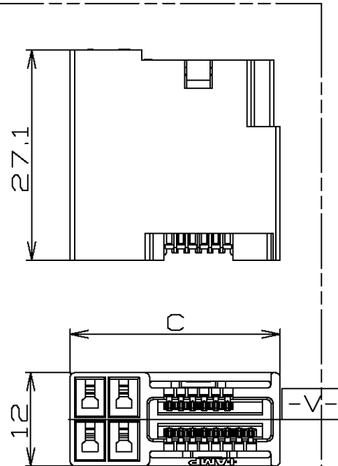
⑥ PLUG ASSEMBLY
