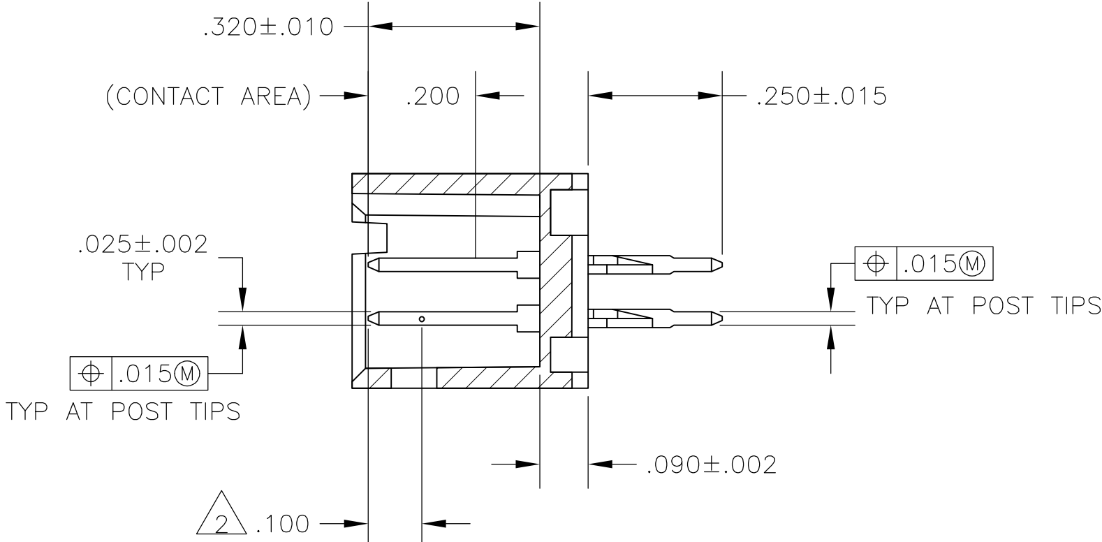
SECTION X-X
