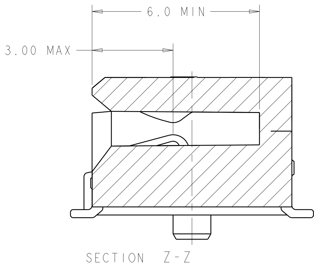
SECTION Z-Z
