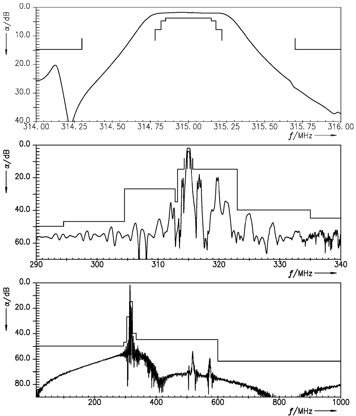
Figure 5: Attenuation.
