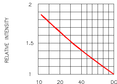
Fig.4 LUMINOUS INTENSITY VS. DUTY CYCLE
