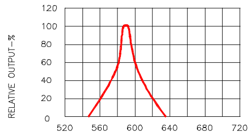
Fig.2 SPECTRAL RESPONSE
