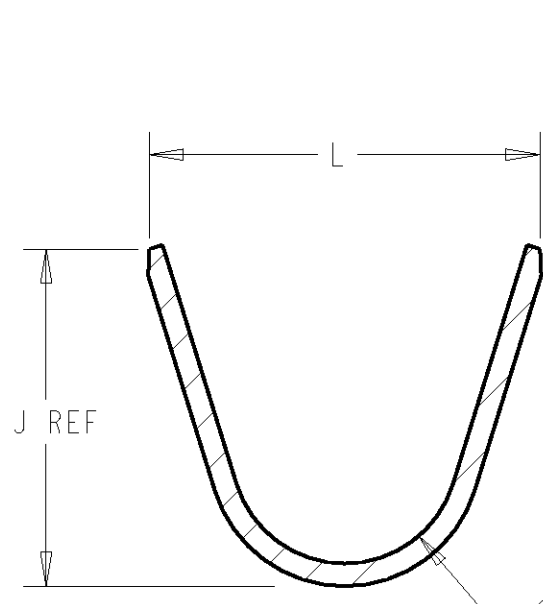
SECTION F-F
