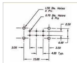
P.C. MOUNTING
