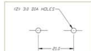
PANEL MOUNT
