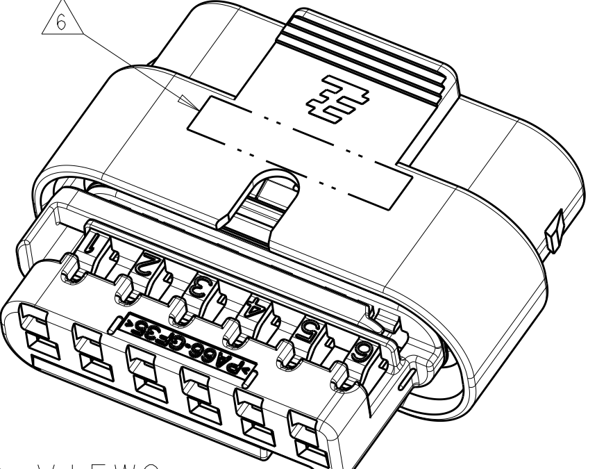
ISOMETRIC VIEWS SCALE 3:1
