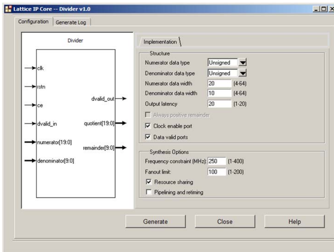
Figure 4-2. Configuration GUI
