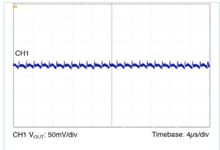
Figure 17 — Output ripple 24V IN , 2.5V OUT at 15A C_{OUT} = 8 \times 100\mu F ceramic
