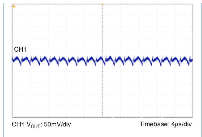
Figure 18 — Output ripple 24V IN , 2.5V OUT at 7.5A C_{OUT} = 8 \times 100\mu F ceramic
