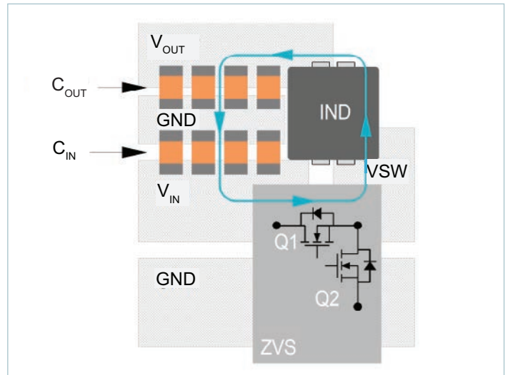
Figure 33 — Recommended component placement and metal routing
