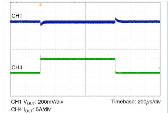
Figure 16 — Transient response 7.5A to 15A, at 5A/μs; 24V IN to 2.5V OUT , C_{OUT} = 8 \times 100\mu F ceramic
