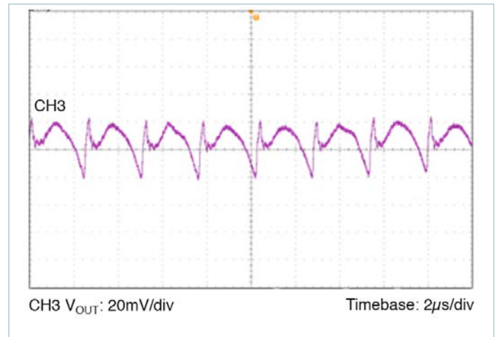
Figure 11 — Output ripple 24V IN , 1.8V OUT at 15A; C OUT = 8 x 100μF ceramic
