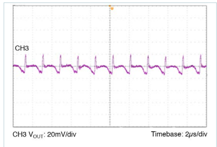
Figure 12 — Output ripple 24V IN , 1.8V OUT at 7.5A; C OUT = 8 x 100μF ceramic
