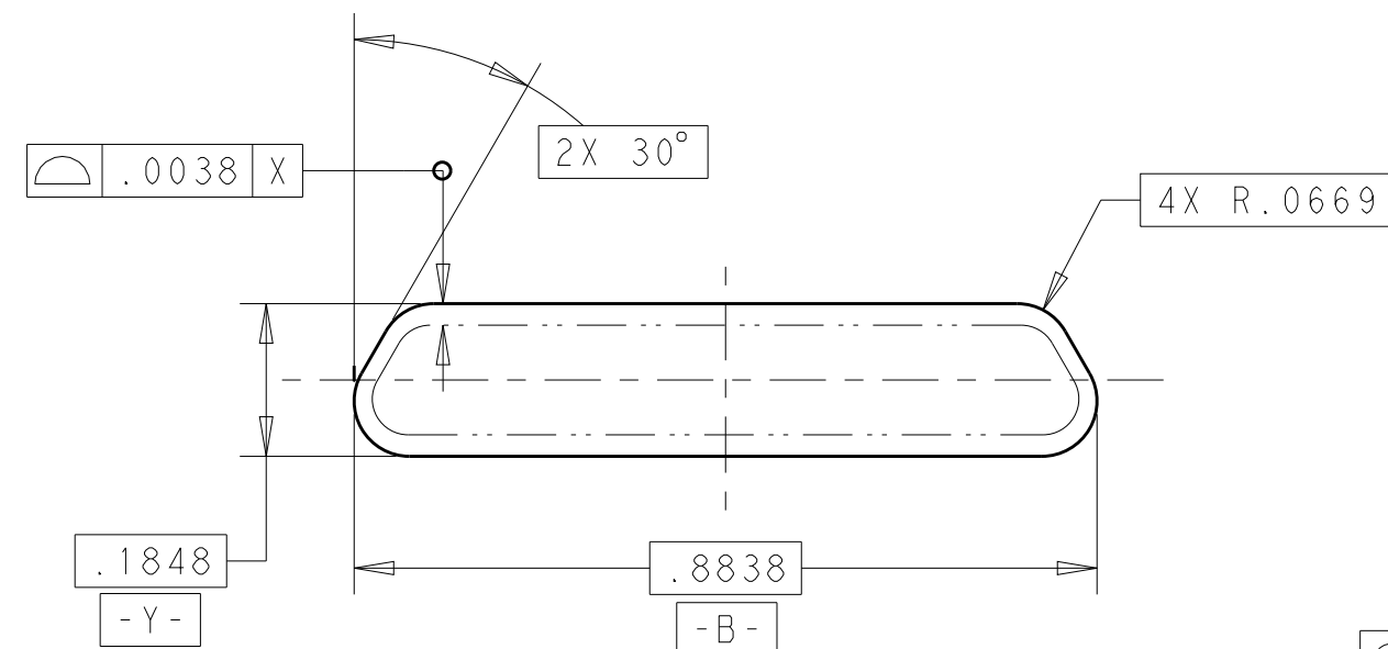
INTERFACE DETAIL
