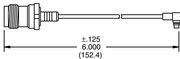
Right Angle MicroMate Plug to RP-TNC Jack 095-680-58000
