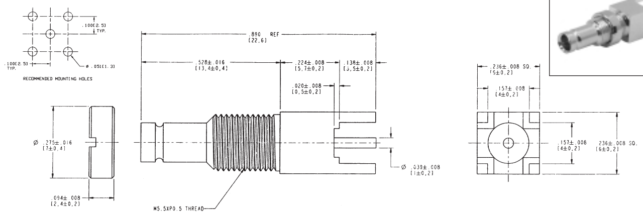
Straight PCB Bulkhead Jack Receptacles 102-692-10
