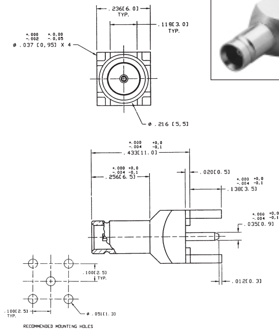
Straight PCB Jack Receptacles 102-692-01 3.5mm Legs (.138)
