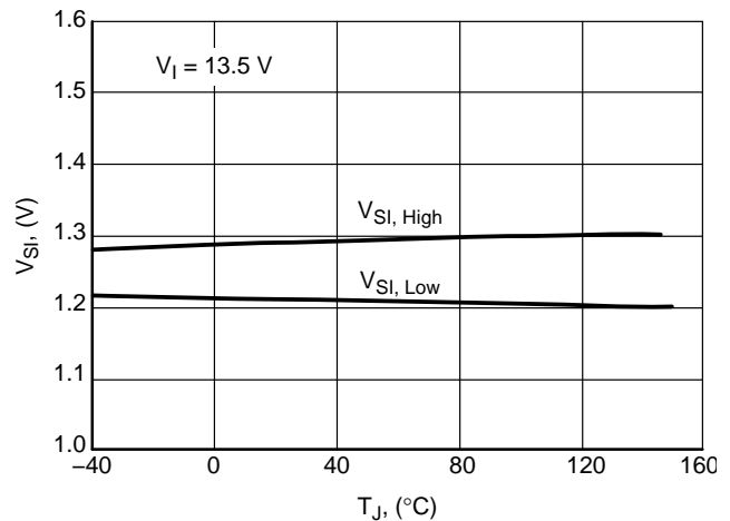
Figure 24. Sense Threshold V_{S1} vs. Temperature T_J
