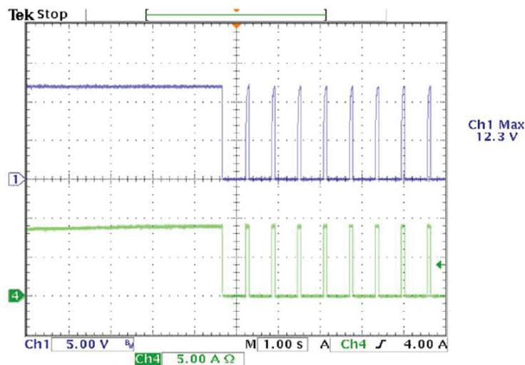
12V Out, 240Vac
