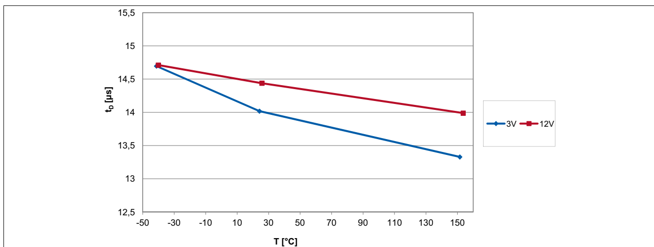
Figure 6-2 Signal Delay Time of the TLE4961-5M over Temperature
