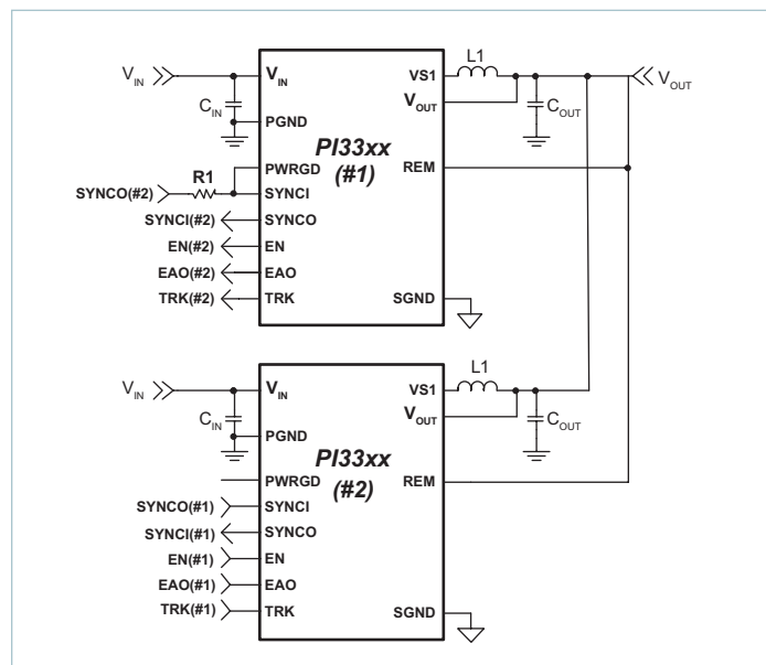
Figure 59 — PI33xx-x0 parallel operation
