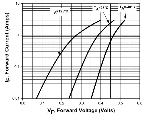
Forward Voltage for CMSH3-40
