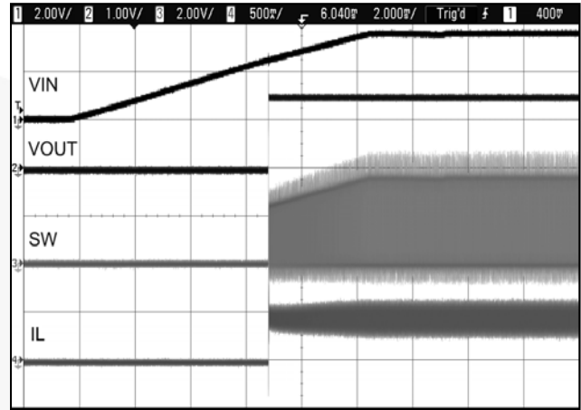
Figure 53. Cold-Start Transient Response from 0 mA to 50 mA in Low-Power Mode
