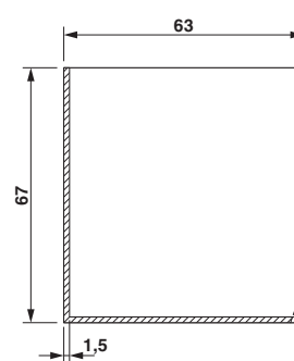
Dimensional drawing
